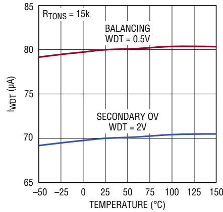
WDT Pin Current vs Temperature
