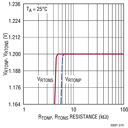
V_{RTONP} , V_{RTONS} vs External Resistance
