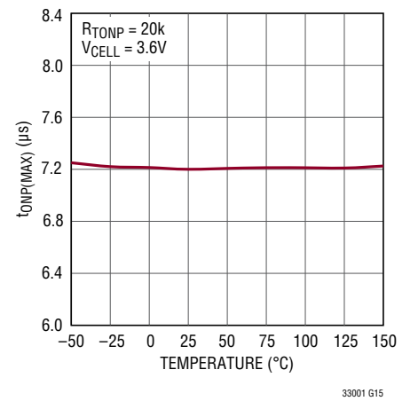
Primary Winding Switch Maximum On-Time vs Temperature
