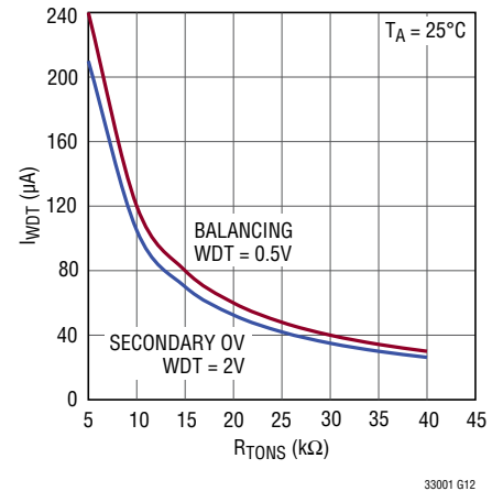
WDT Pin Current vs R_{TONS}
