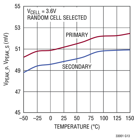
Peak Current Sense Threshold vs Temperature
