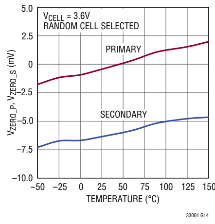
Zero Current Sense Threshold vs Temperature
