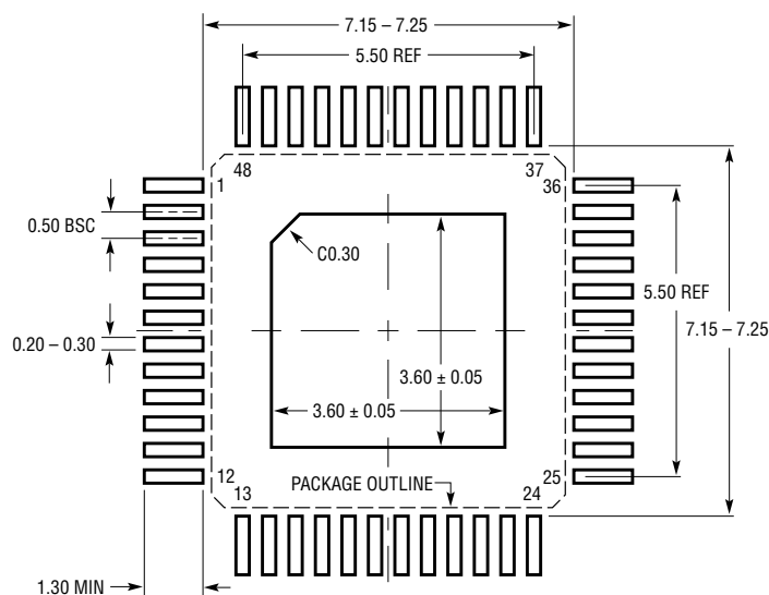
LXE Package 48-Lead Plastic Exposed Pad LQFP (7mm × 7mm) (Reference LTC DWG # 05-08-1832 Rev B)
