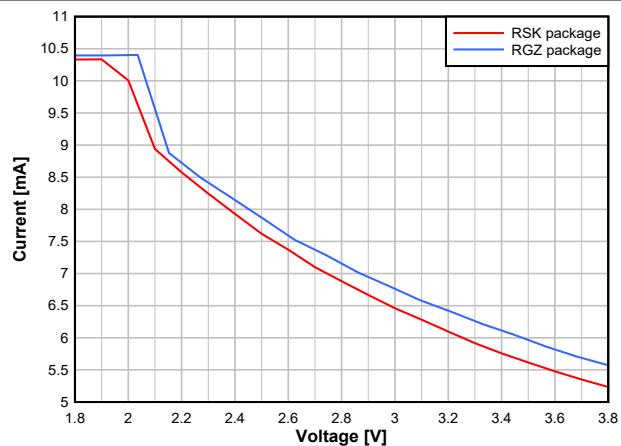
Figure 8-9. RX Current vs. Supply Voltage (VDD5) (BLE 1 Mbps, 2.44 GHz)
