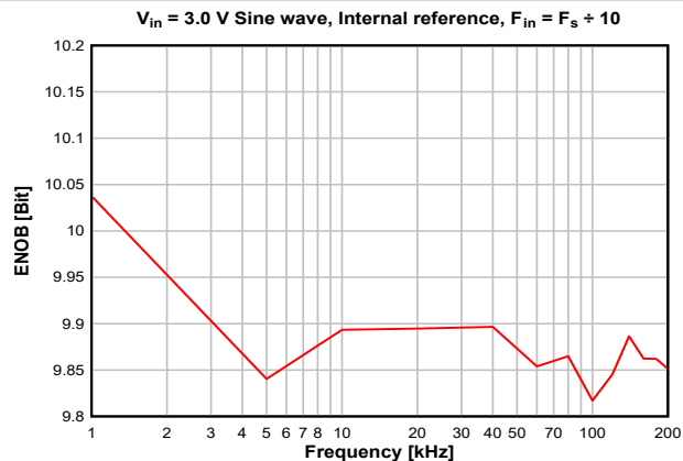
Figure 8-36. ENOB vs. Sampling Frequency
