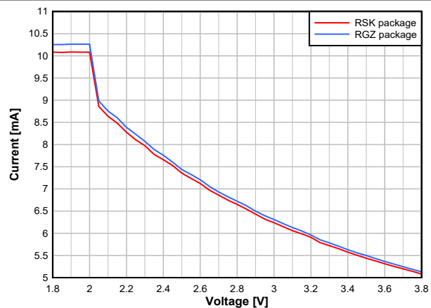
Figure 8-8. RX Current vs. Supply Voltage (VDD5) (50 kbps, 868.3 MHz)
