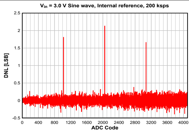
Figure 8-38. DNL vs. ADC Code
