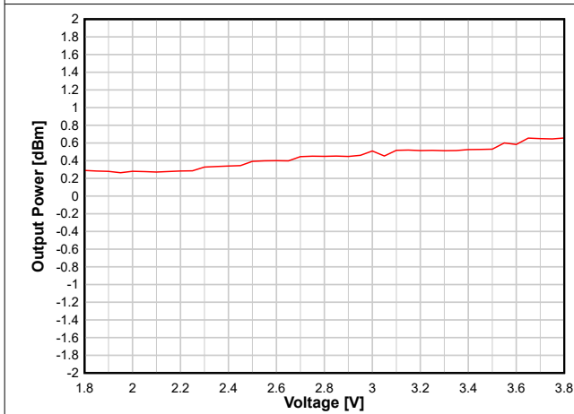
Figure 8-18. Output Power vs. Supply Voltage (VDDS) (BLE 1 Mbps, 2.44 GHz, 0dBm)
