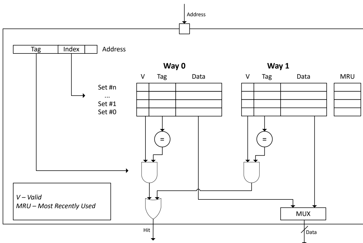
Figure 8: Cache overview
