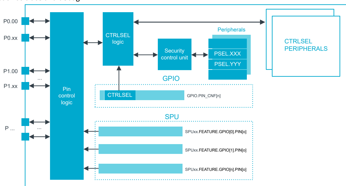
Figure 62: Pin access using CTRLSEL
