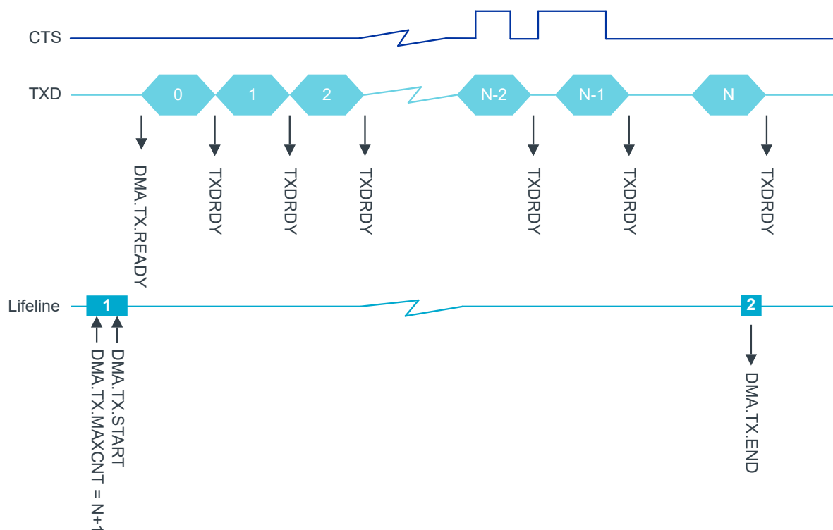
Figure 159: UARTe transmission
