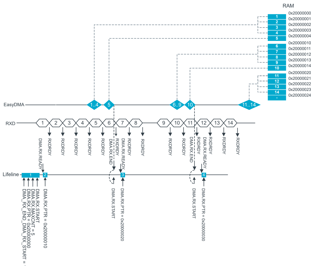
Figure 160: UARTE reception
