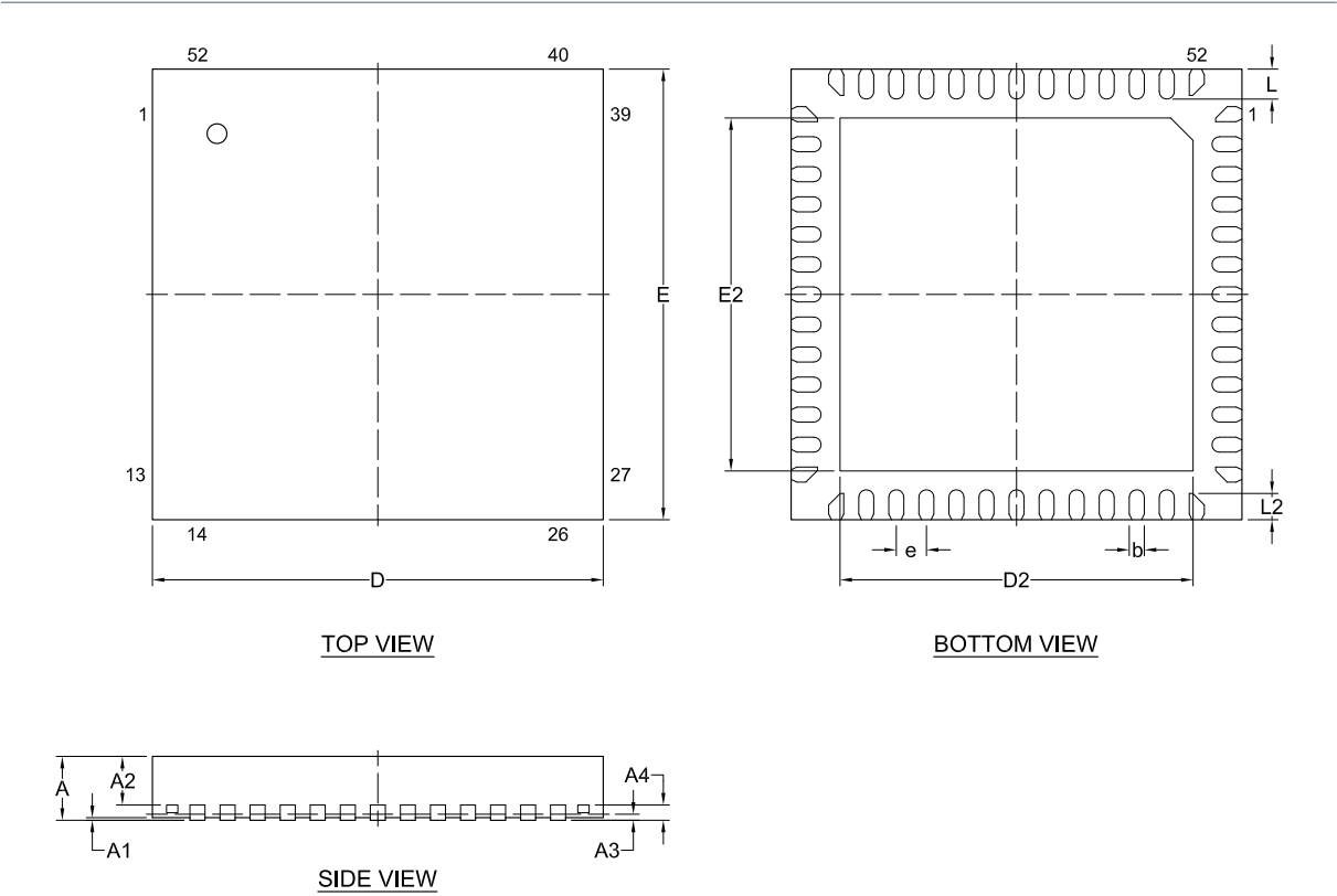
Figure 178: QFN52 6x6 mm package
