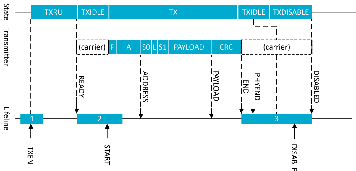
Figure 115: Transmit sequence
