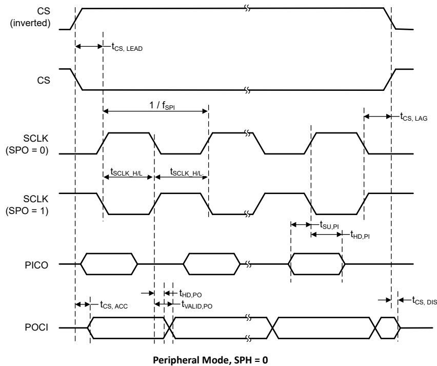
Figure 7-3. SPI Timing Diagram—Peripheral Mode, SPH = 0
