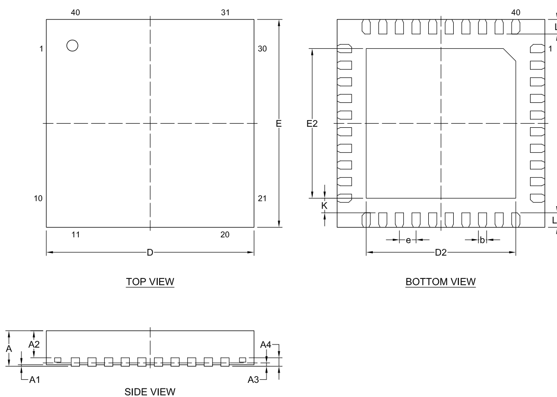
Figure 176: QFN40 5x5 mm package
