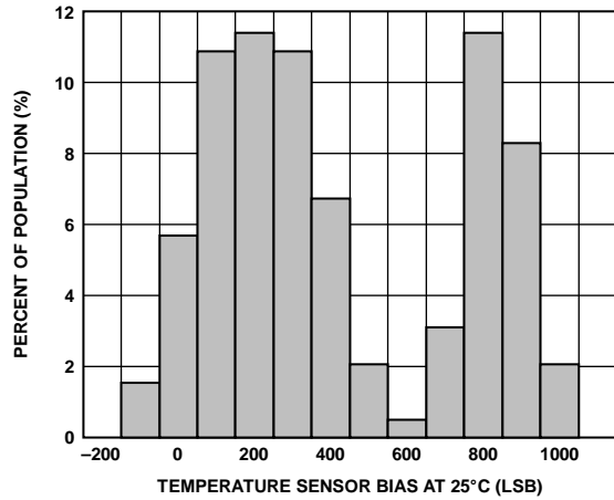
Figure 26. Temperature Sensor Response at 25°C, V_S = 2 V
