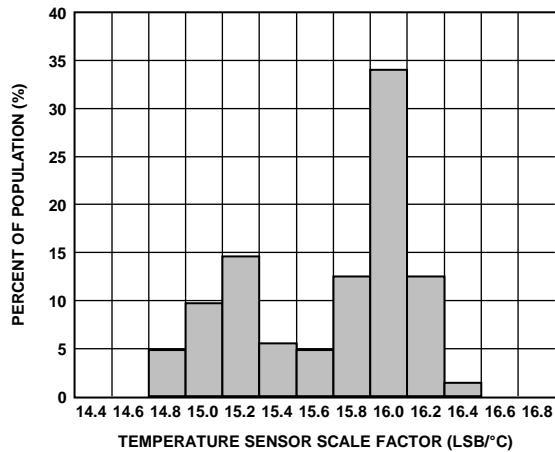
Figure 27. Temperature Sensor Scale Factor, V_S = 2 V
