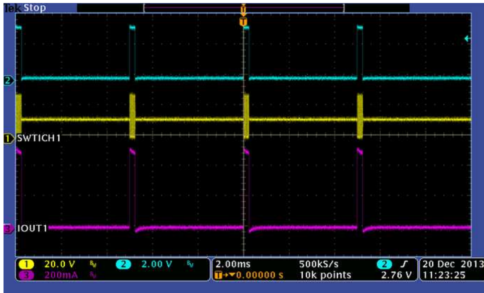
Figure 8. PWM Dimming, f_{PWM} = 200 \text{ Hz} , Duty Cycle = 5%
