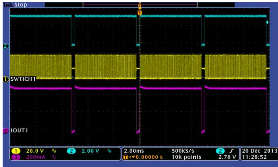
Figure 9. PWM Dimming, f_{PWM} = 200 \text{ Hz} , Duty Cycle = 95%
