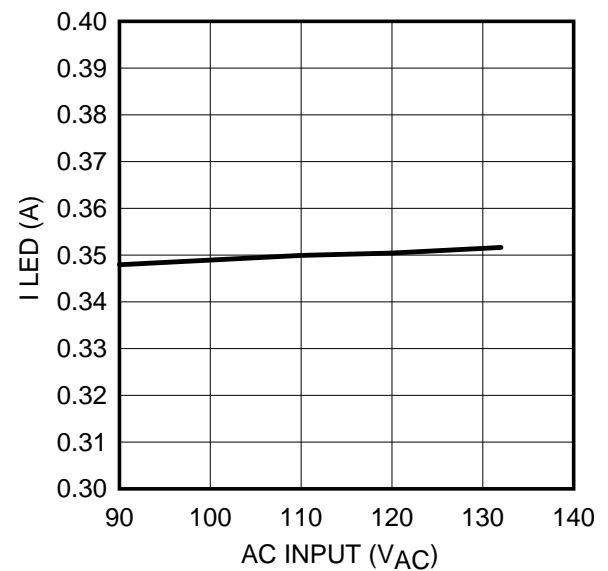
Figure 7. Line Regulation
