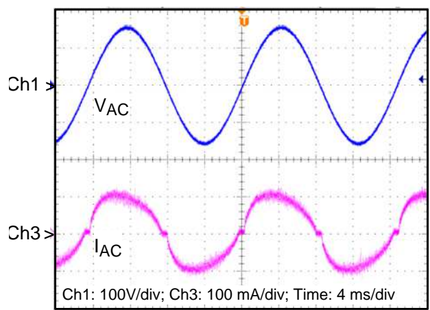
Figure 13. Input Voltage and Input Current (120VAC)
