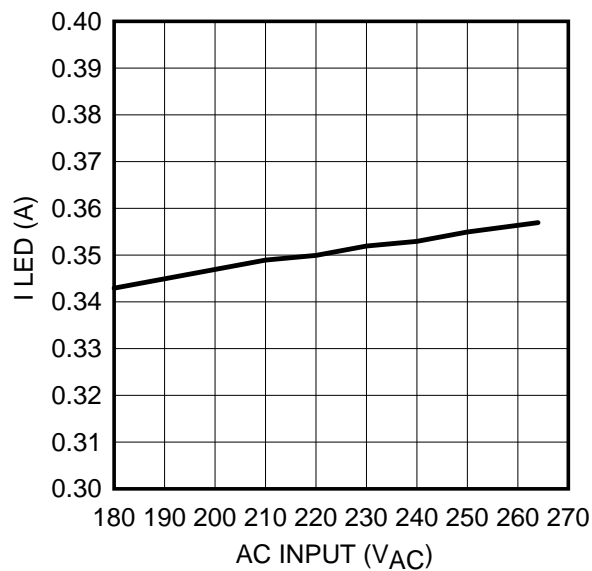
Figure 6. Line Regulation
