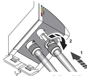
Figure 17 B-FOC connection
