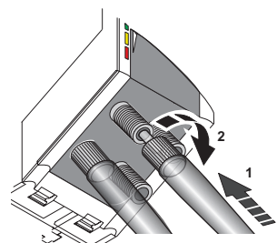
Figure 16 F-SMA connection
