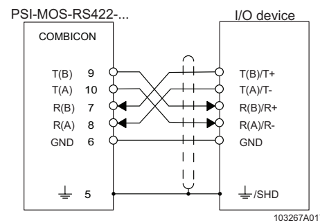
Figure 14 Connection to RS-422/RS-485 4-wire
