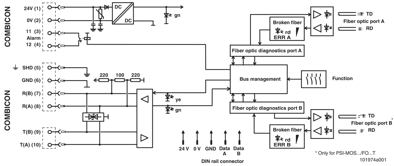
Figure 1 Block diagram
