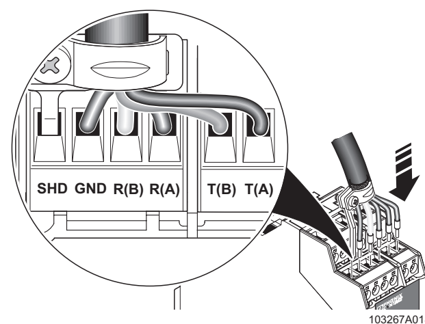
Figure 11 Shield connection
