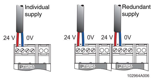
Figure 10 Individual/redundant supply
