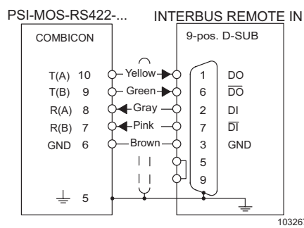
Figure 13 Connection to INTERBUS REMOTE IN
