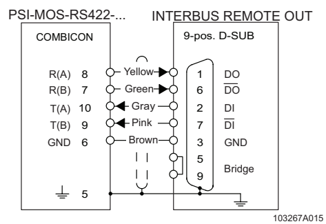
Figure 12 Connection to INTERBUS REMOTE OUT
