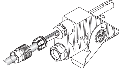
Figure 27 Bus connector
