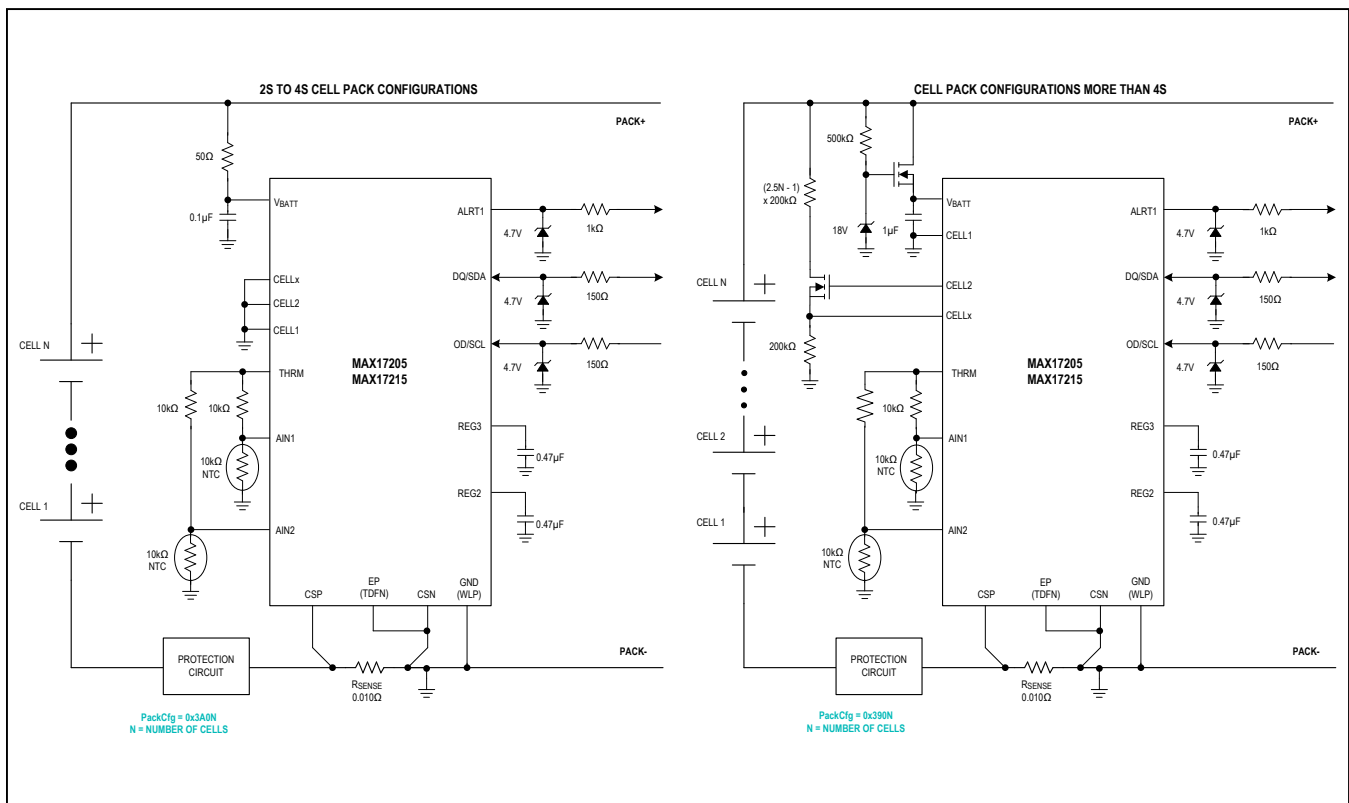
Figure 2. Multicell Schematics
