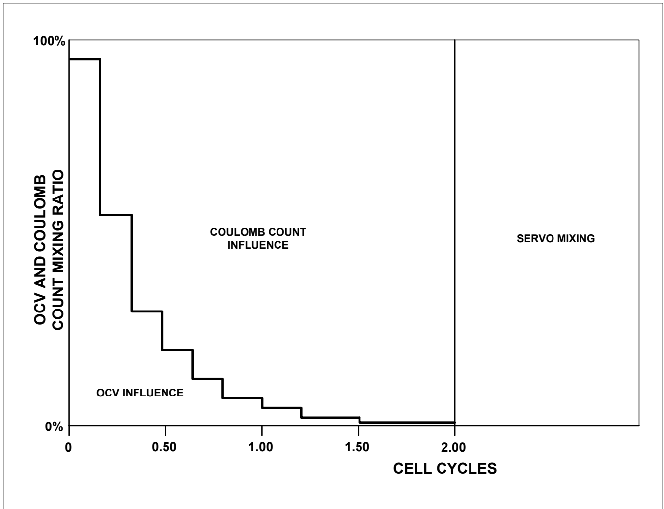
Figure 17. Voltage and Coulomb Count Mixing
