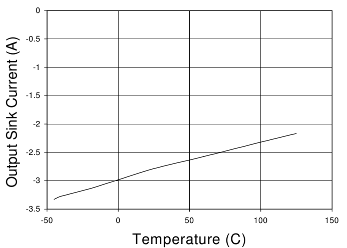
Fig. 28 Output Sink Current vs. Temperature V_{SUPPLY} = 15V
