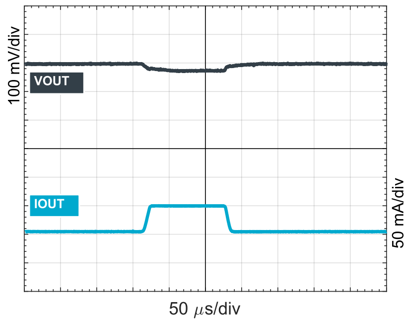
Figure 40: VINLDO = 3.8 V; VOUTLDO = 1.8 V; LDO load transient
