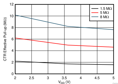
Figure 6-5. CTR Internal Pull-Up Resistor (if Configured) Across VDD
