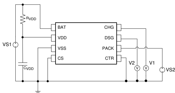
Figure 8-2. Test Circuit 2
