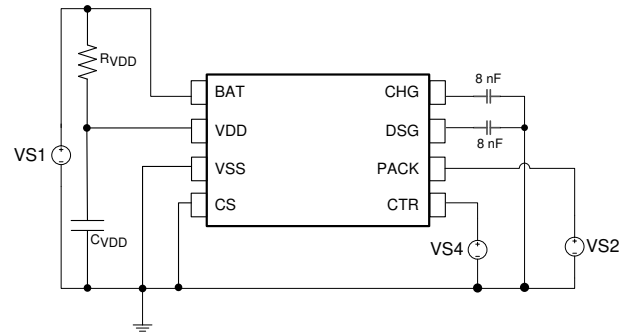
Figure 8-4. Test Circuit 4
