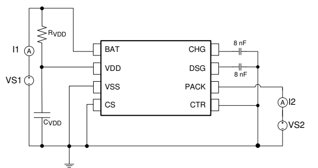
Figure 8-1. Test Circuit 1
