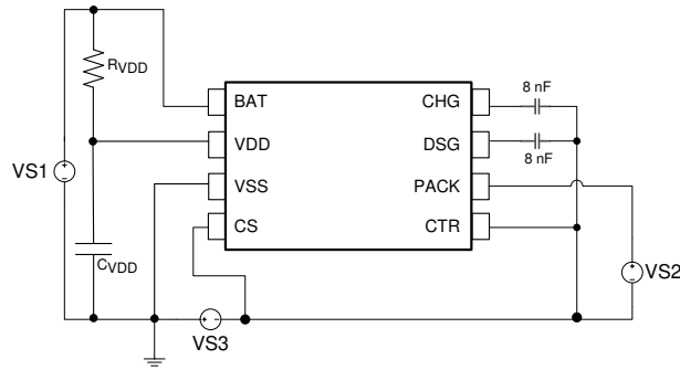
Figure 8-3. Test Circuit 3
