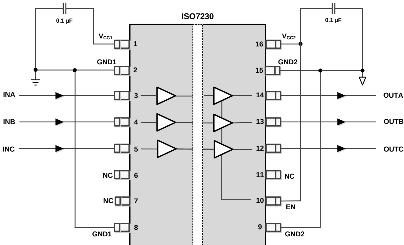
Figure 17. Typical ISO7230 Circuit Hook-up
