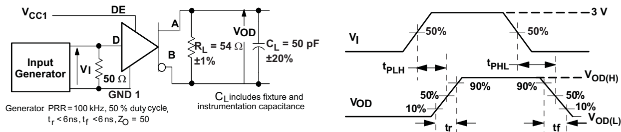
Figure 14. Driver Switching Test Circuit and Voltage Waveforms
