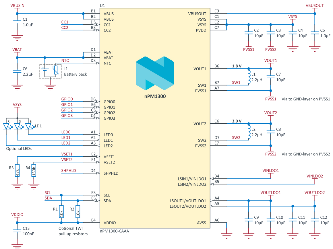
Figure 55: WLCSP schematic
