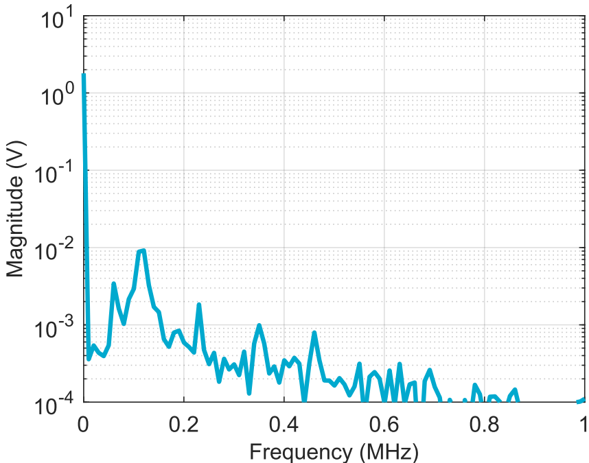
Figure 32: V_{OUT} = 1.8\text{ V} : FFT 50 mA: PFM
