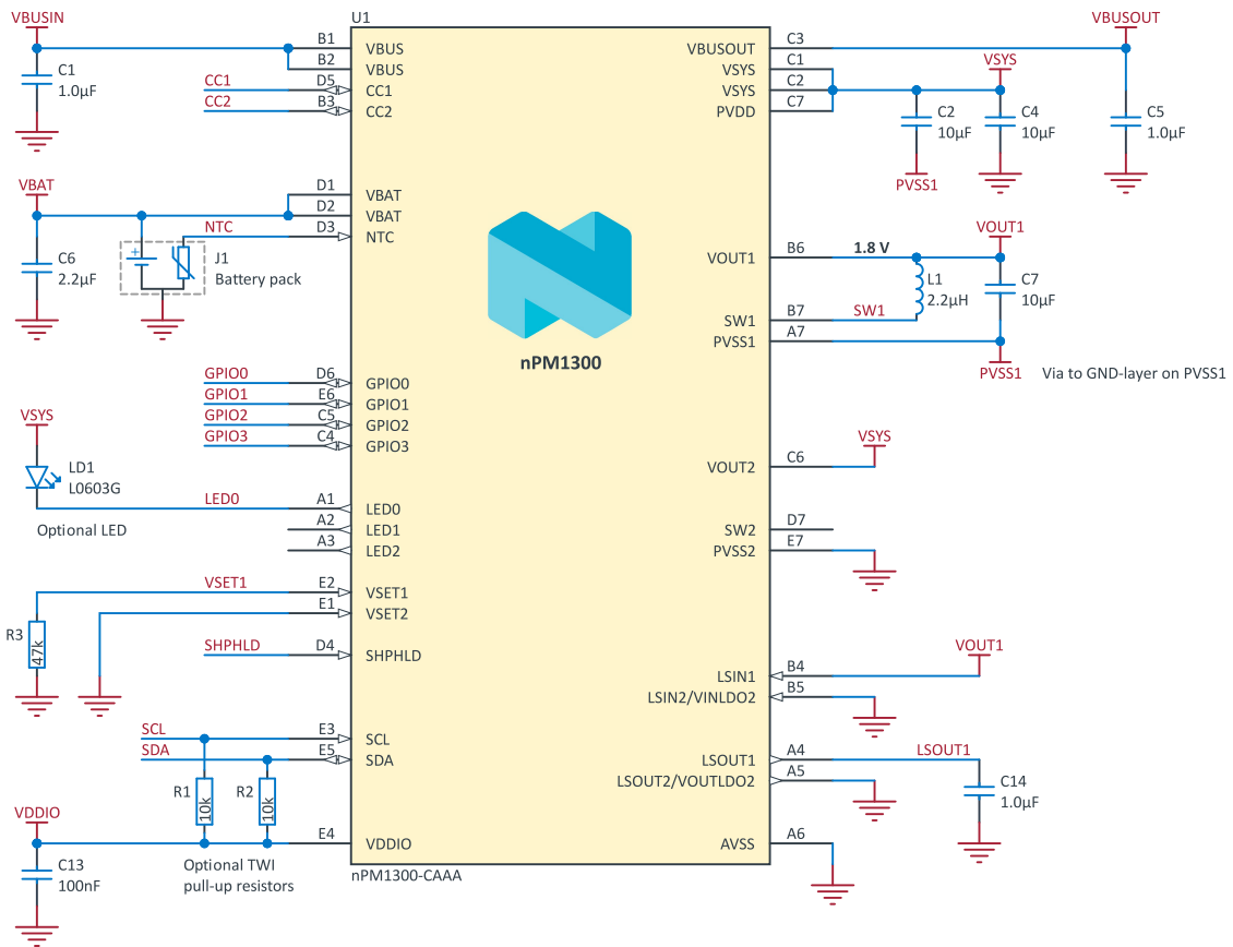
Figure 57: WLCSP schematic
