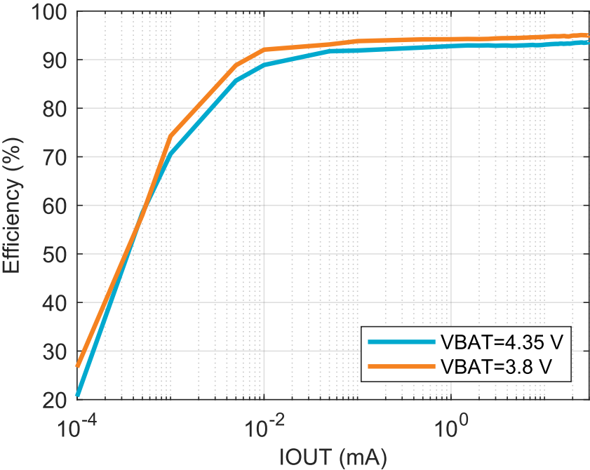
Figure 30: VOUT = 3.3 V: Hysteretic efficiency
