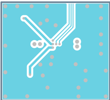
Figure 68: Mid layer 2 WLCSP
