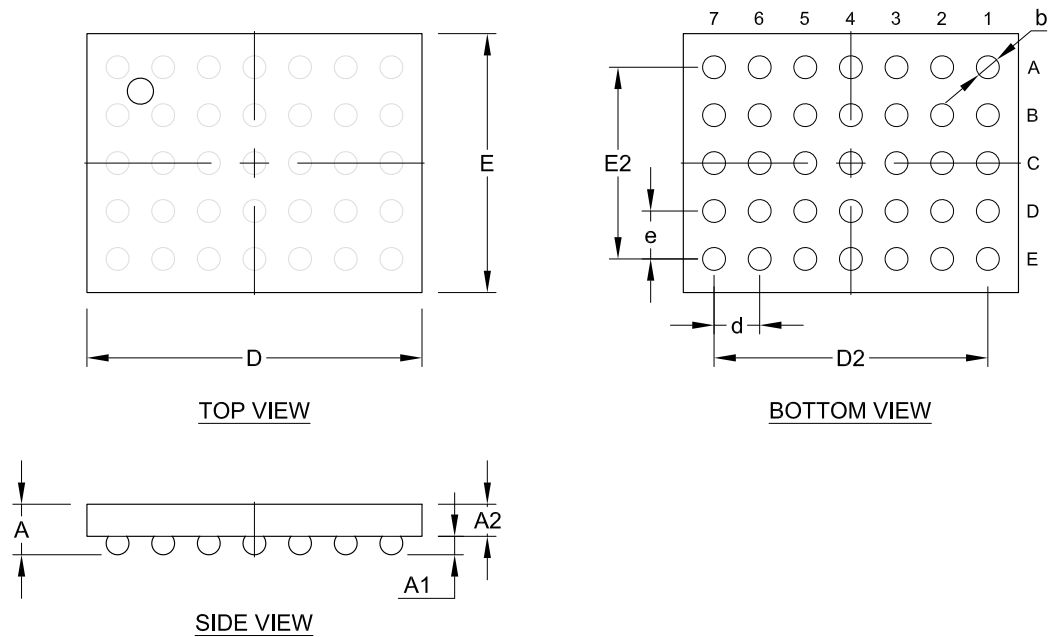
Figure 53: WLCSP 2.3775x3.0775 mm package
