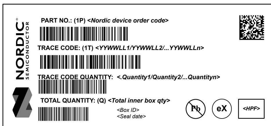
Figure 73: Inner box label
