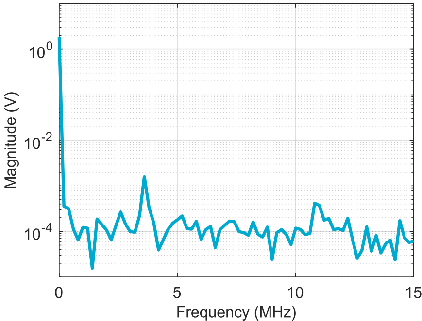
Figure 33: V_{OUT} = 1.8\text{ V} ; FFT 100 mA; PWM: clock = 3.6 MHz
