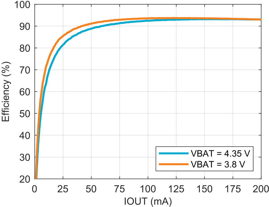
Figure 26: VOUT = 3.3 V: PWM efficiency
