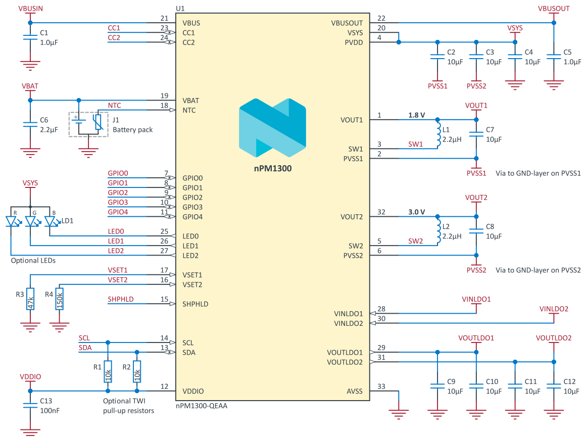
Figure 54: QFN schematic
