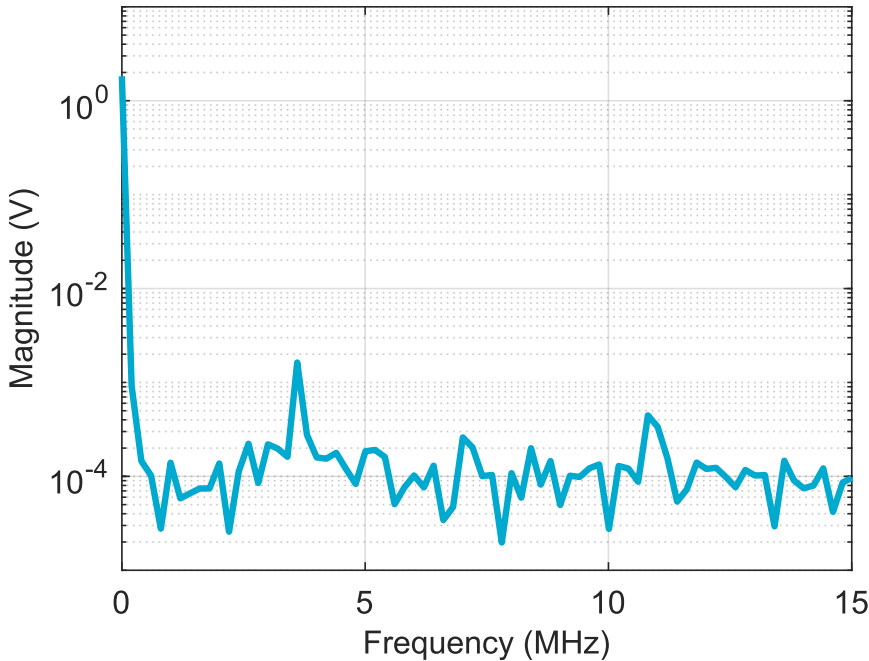
Figure 34: V_{OUT} = 1.8\text{ V} ; FFT 200 mA; PWM: clock = 3.6 MHz
