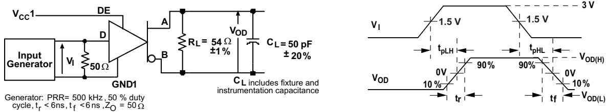
Figure 17. Driver Switching Test Circuit and Waveforms
