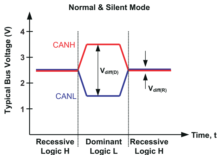
Figure 8-1. Bus States (Physical Bit Representation)
