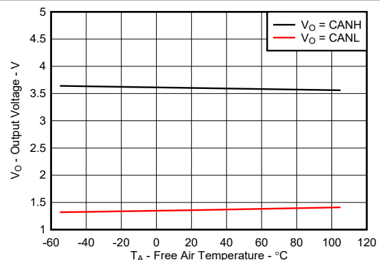
Figure 6-6. Driver Output Voltage vs Free-Air Temperature
