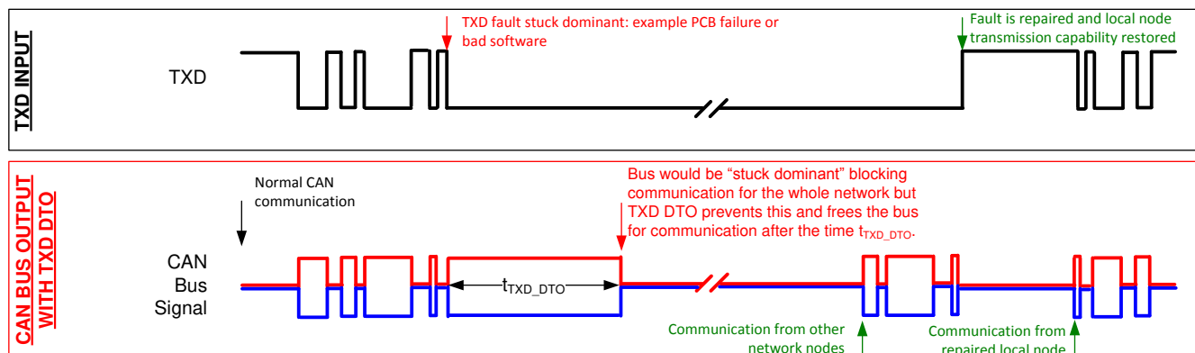
Figure 8-3. Example Timing Diagram for Devices With TXD DTO
