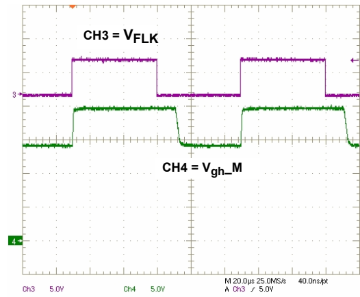
FIGURE 16. GPM WAVEFORM
