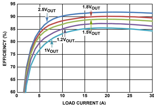
FIGURE 7. EFFICIENCY vs LOAD CURRENT (PARALLEL SINGLE OUTPUT, AS SHOWN IN Figure 19 AT 12V_{\text{IN}}/500\text{kHz} )
