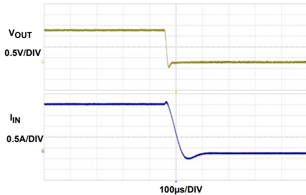
FIGURE 17. SHORT CIRCUIT AT 15A
