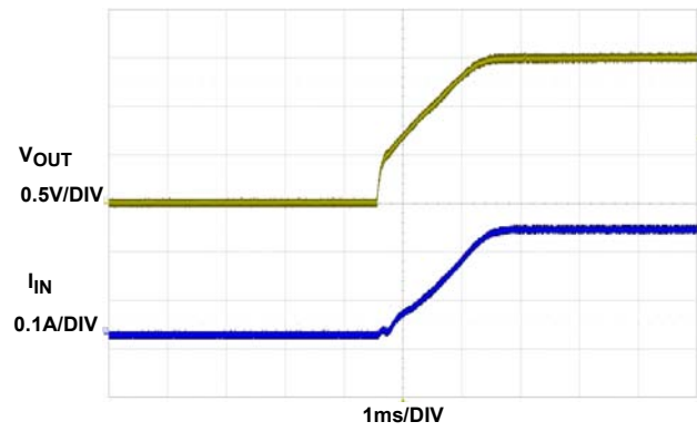
FIGURE 15. START-UP AT 15A
