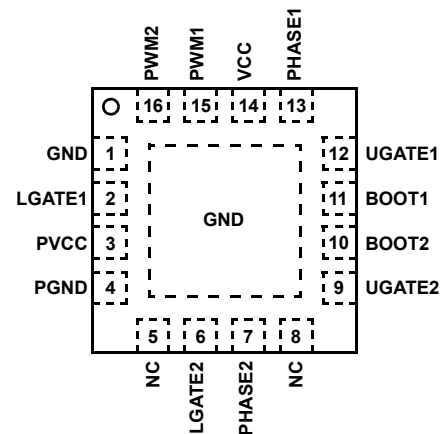
ISL6614CR, ISL6614CRZ, ISL6614IR, ISL6614IRZ (16 LD QFN) TOP VIEW
