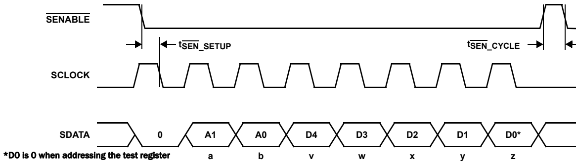
FIGURE 35. SERIAL TIMING
