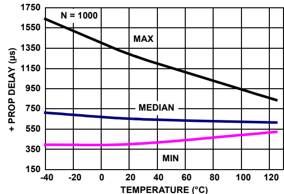
FIGURE 38. ISL28197 POSITIVE PROP DELAY vs TEMPERATURE 50% TO 20%, V_+ = 5V
