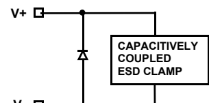
CIRCUIT 4
