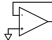
FIGURE 43. PREVENTING OSCILLATIONS IN UNUSED CHANNELS
