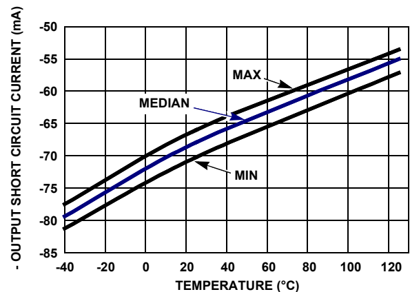
FIGURE 41. - OUTPUT SHORT CIRCUIT CURRENT vs TEMPERATURE V_{IN} = -2.5V, R_L = 10, V_+, V_- = \pm 2.5V
