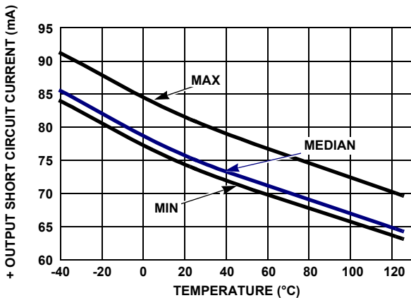
FIGURE 40. + OUTPUT SHORT CIRCUIT CURRENT vs TEMPERATURE V_{IN} = -2.5V, R_L = 10, V_+, V_- = \pm 2.5V
