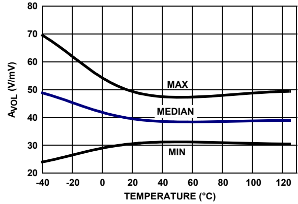
FIGURE 33. A_{VOL} vs TEMPERATURE, R_L = 1k, V_+, V_- = \pm 2.5V, V_O = -2V \text{ TO } +2V
