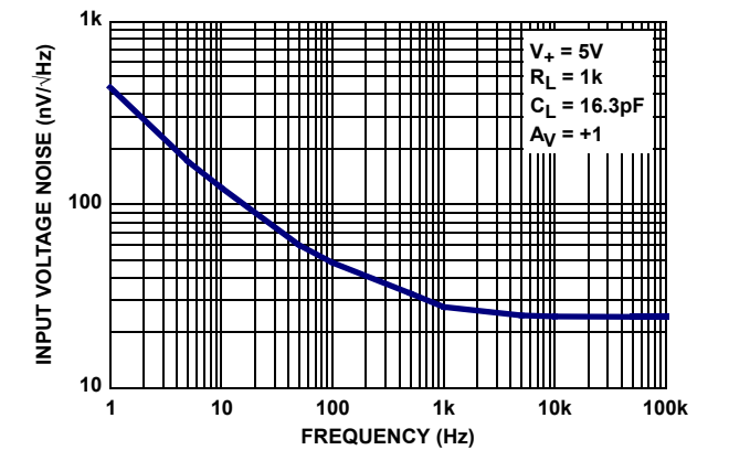
FIGURE 12. INPUT VOLTAGE NOISE DENSITY vs FREQUENCY
