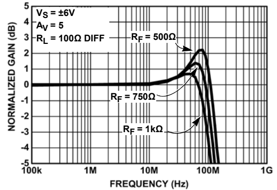
FIGURE 7. DIFFERENTIAL FREQUENCY RESPONSE WITH VARIOUS R_F (LOW BIAS MODE)
