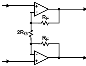
FIGURE 21. DRIVERS WIRED FOR DIFFERENTIAL INPUT
