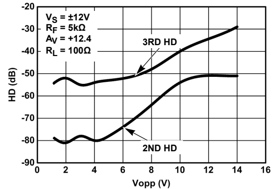
FIGURE 10. 3.75MHz 2ND AND 3RD HARMONIC DISTORTION vs OUTPUT VOLTAGE (HALF POWER MODE)
