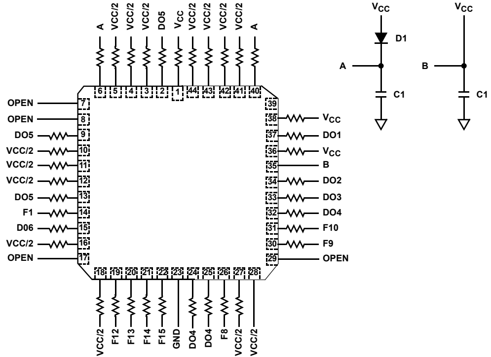
MR82C37A CLCC
