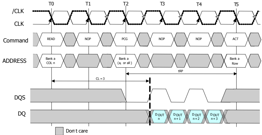
Figure19 : Read to Precharge (BL=4)
