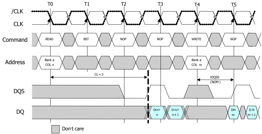
Figure18 : Read to write terminate (BL=4,8 or 16)
