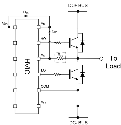
Figure 10: V_S resistor
