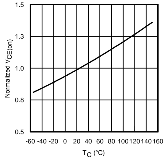
Fig. 18 - Normalized Typ. V_{\text{CE(on)}} vs. Junction Temperature I_C = 33\text{A} , V_{\text{GE}} = 15\text{V}
