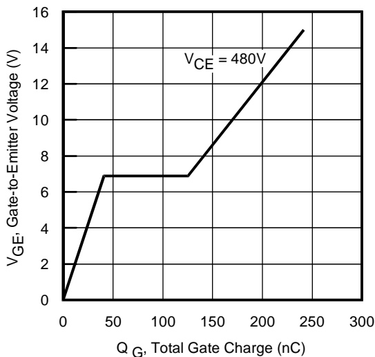
Fig. 17 - Typical Gate Charge vs. V_{\text{GE}} I_{\text{CE}} = 33\text{A}
