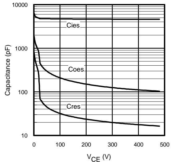
Fig. 16 - Typ. Capacitance vs. V_{\text{CE}} V_{\text{GE}} = 0\text{V} ; f = 1\text{MHz}
