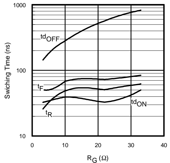
Fig. 14 - Typ. Switching Time vs. R_G T_J = 125^\circ\text{C} ; L = 200\mu\text{H} ; V_{\text{CE}} = 390\text{V} ; I_{\text{CE}} = 33\text{A} ; V_{\text{GE}} = 15\text{V} Diode clamp used: 30ETH06 (See C.T.3)
