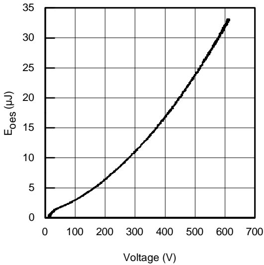
Fig. 15 - Typ. Output Capacitance Stored Energy vs. V_{\text{CE}}
