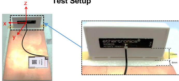
Test Setup
