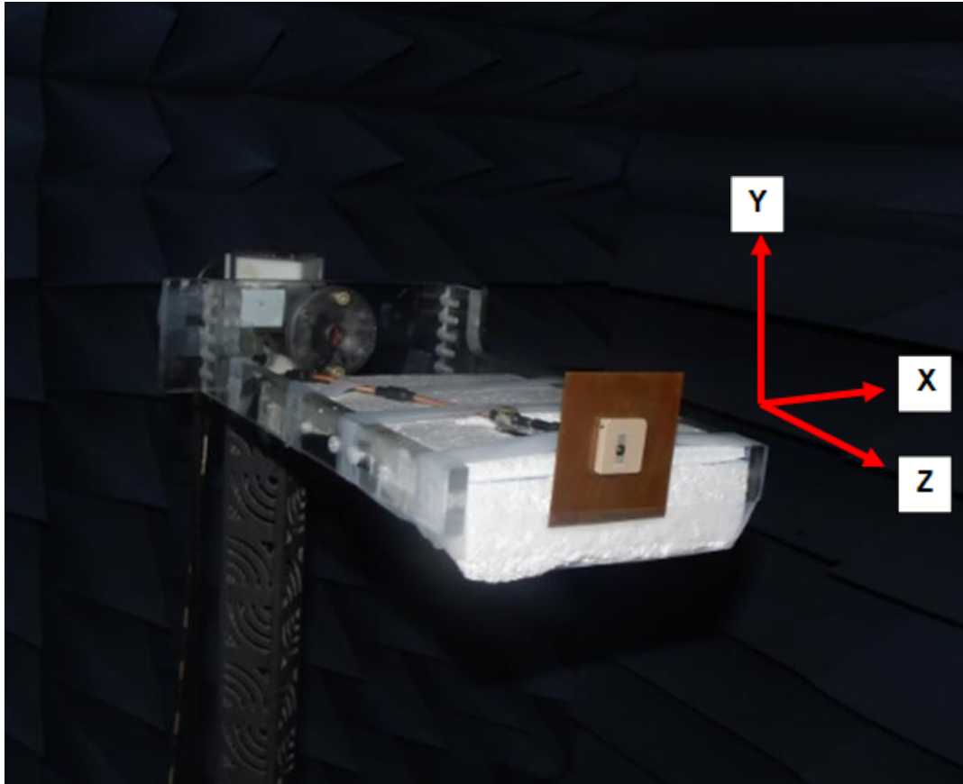
The antenna radiation pattern measurement setup as shown above
