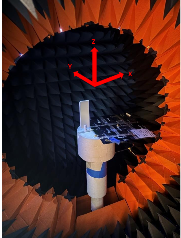
Chamber Set up Bent on the Edge of a 30x30cm Ground Plane
