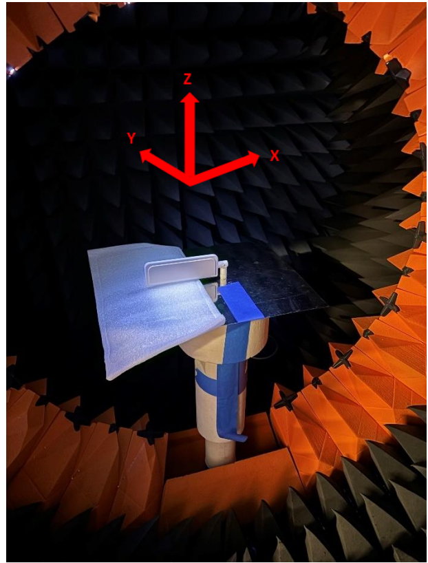
Chamber Set up Bent in the Centre of a 30x30cm Ground Plane
