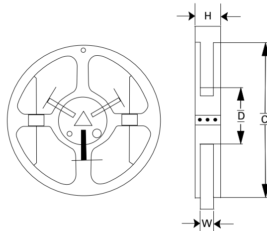
Reel Specifications
