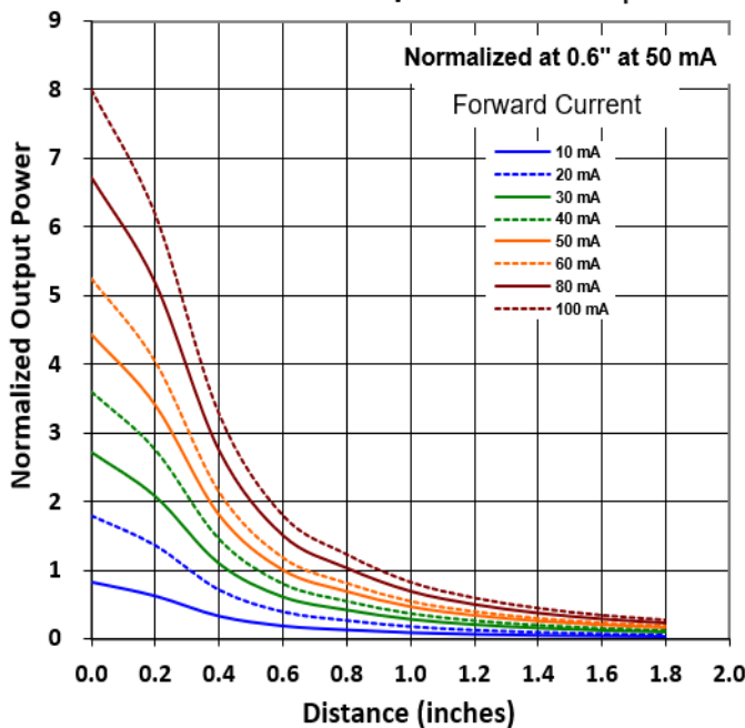
Distance vs Output Power vs I_F
