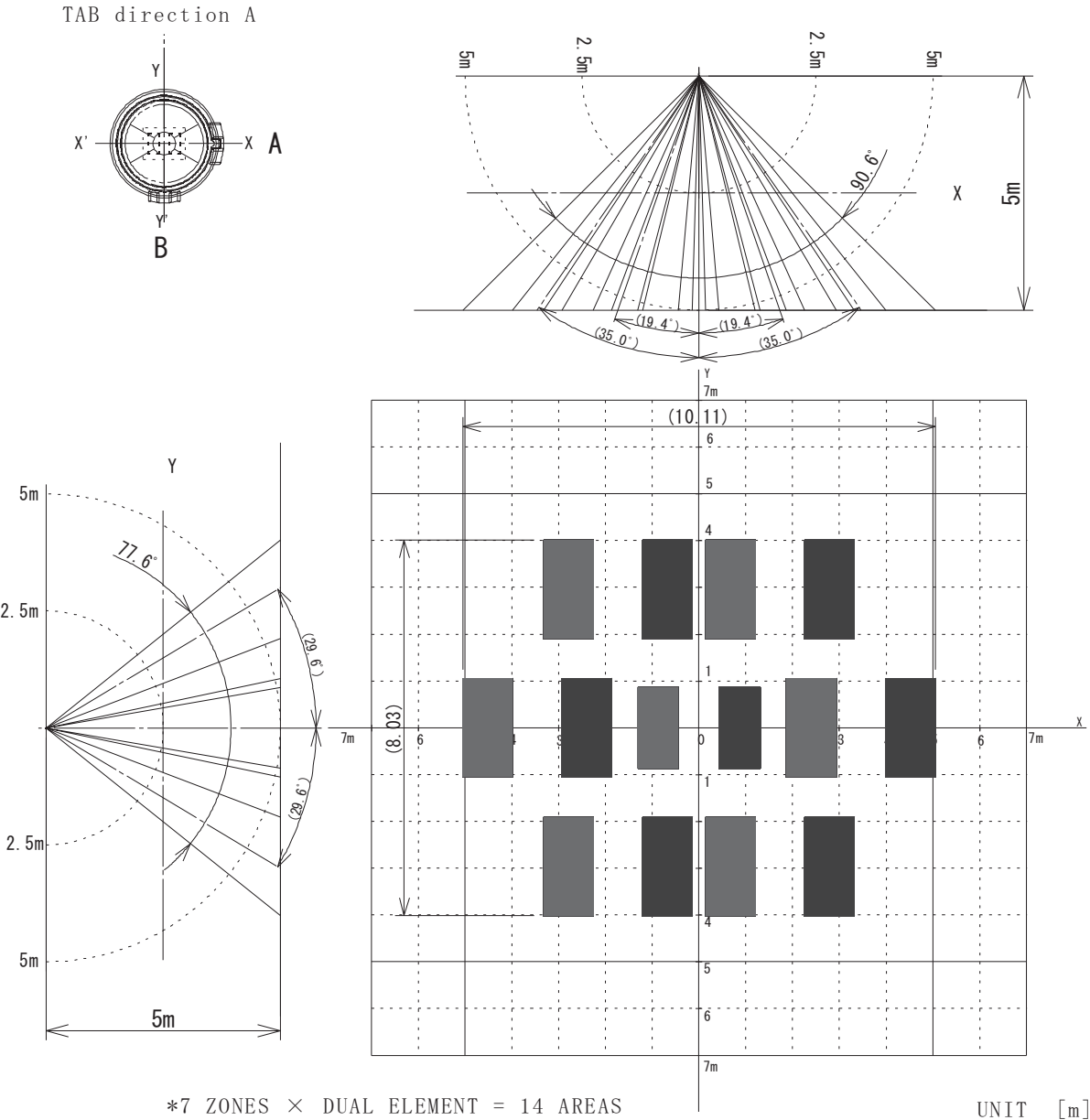
Figure 17. The ZNCL10R Dual-Element Lens Specification, Tab Direction A
