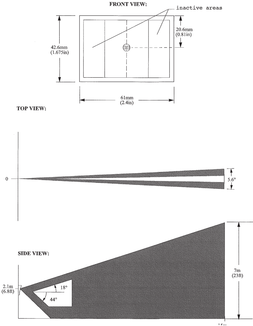
Figure 33. ZVB12GIV1 Lens Specification
