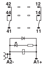
DC coils
