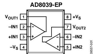
Figure 1. 8-Lead SOIC_N
