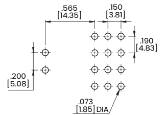
P.C.MOUNTING
