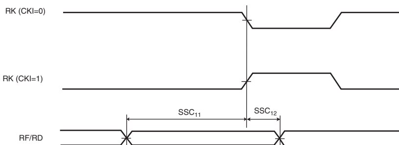
Figure 46-23: SSC Receiver, RK in ouput and RF in Input
