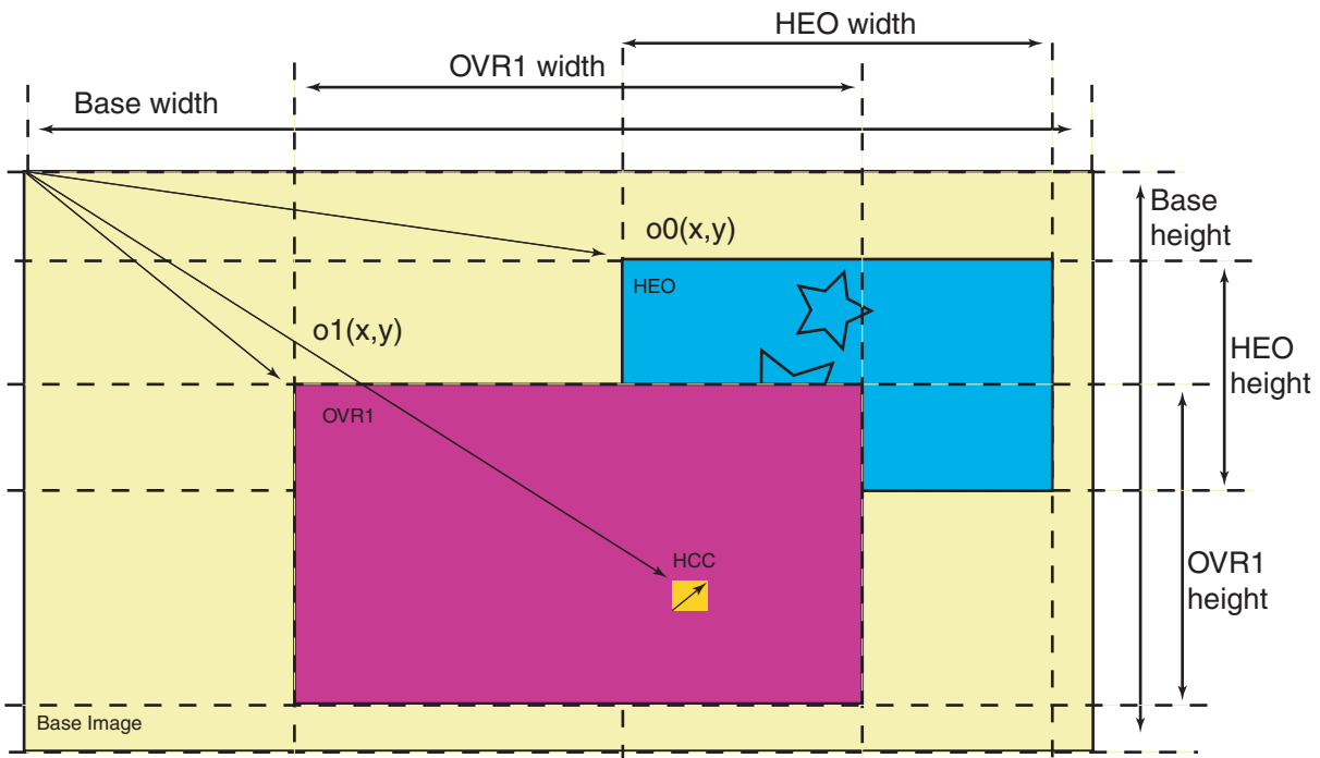
Figure 45-6: Overlay Example with two different video prioritization algorithms
