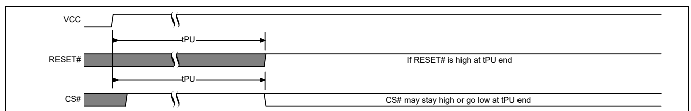
Figure 137 Reset high at the end of POR
