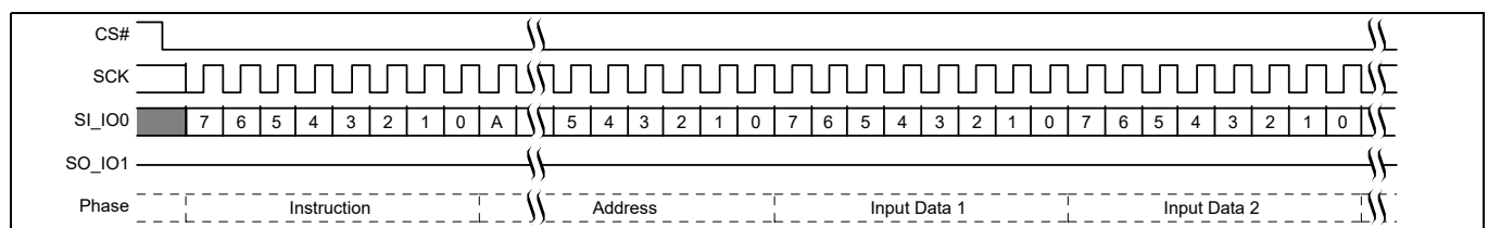
Figure 77 Page Program (PP 02h or 4PP 12h) command sequence [43]
