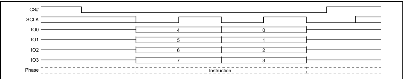
Figure 102 Global IBL Lock (GBL) command sequence QPI mode
