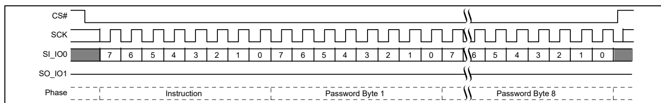
Figure 117 Password Program (PASSP) command sequence
