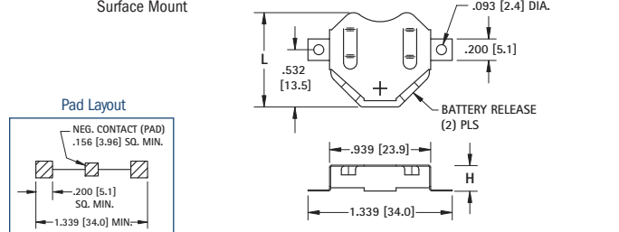
Surface Mount
