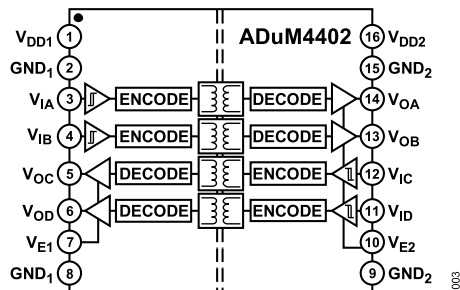
Figure 3. ADuM4402
