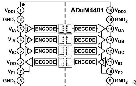
Figure 2. ADuM4401
