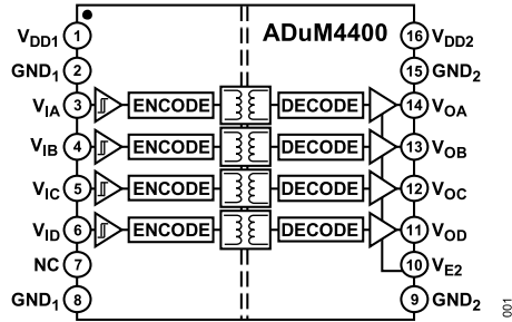
Figure 1. ADuM4400
