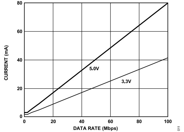
Figure 11. Typical ADuM4400 V DD1 Supply Current vs. Data Rate for 5 V and 3.3 V Operation
