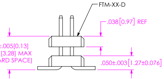
FIG 2 MW-10-03-X-D-120-073 SHOWN (DIFFERENT AS SHOWN, OTHERWISE SAME AS FIG 1)
