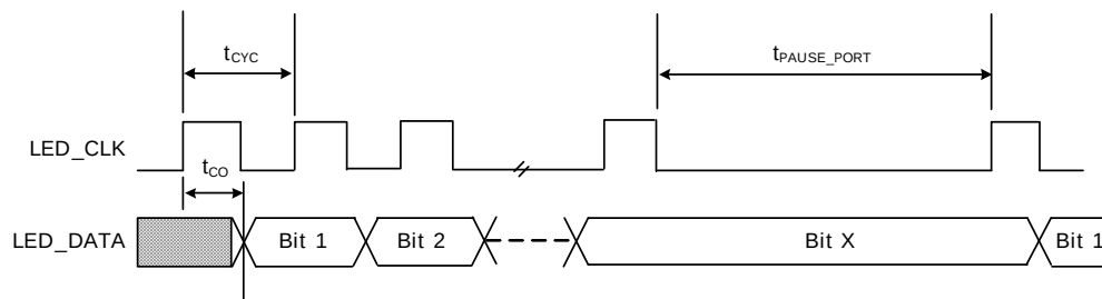
Figure 93 • Basic Serial LED Timing
