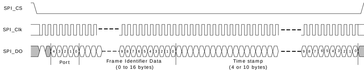
Figure 67 • Serial Time Stamp/Frame Signature Output
