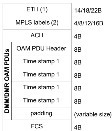
Figure 65 • RFC6374 DMM/DMR OAM PDU Format
