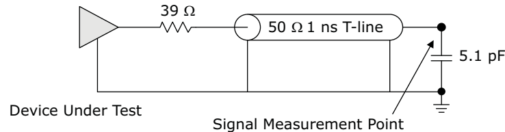
Figure 91 • Test Circuit for Recovered Clock Output Signals
