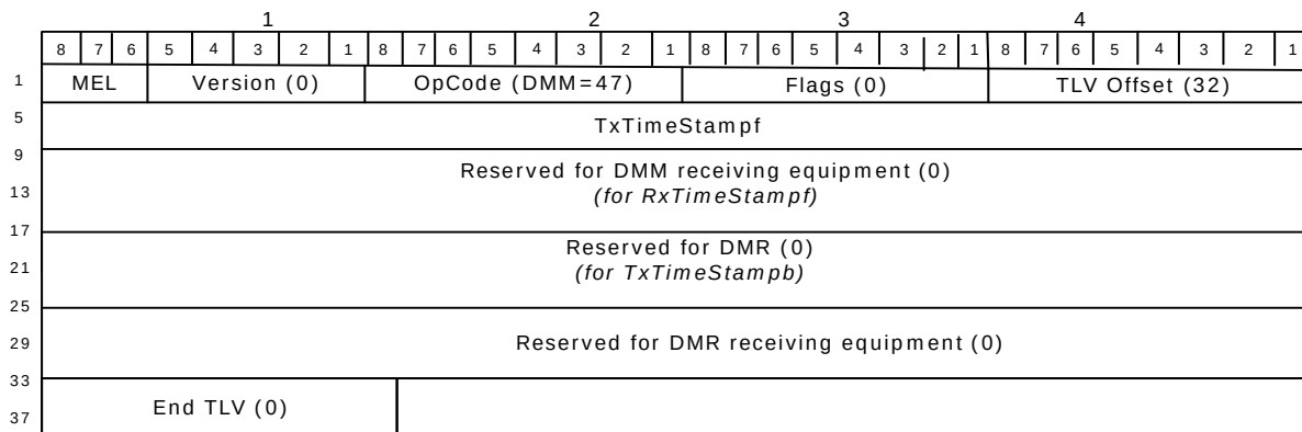
Figure 38 • Y.1731 DMM PDU Format
