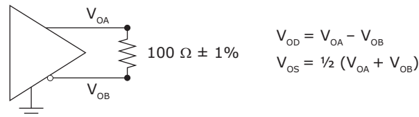
Figure 86 • SGMII DC Transmit Test Circuit
